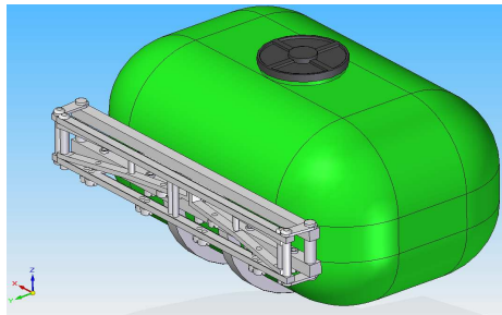
Figure 2. Sprayer installation assembly model [1]
