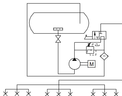
Figure 1. Schematic representation of sprayer installation components
