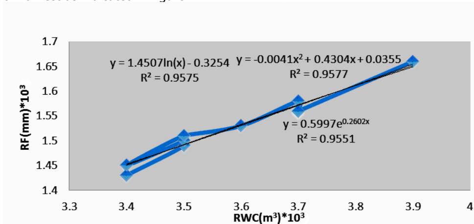
Figure 2. Average rainfall depth (RF) and rainwater (RWC) harvest from roof plan size (250m²)
