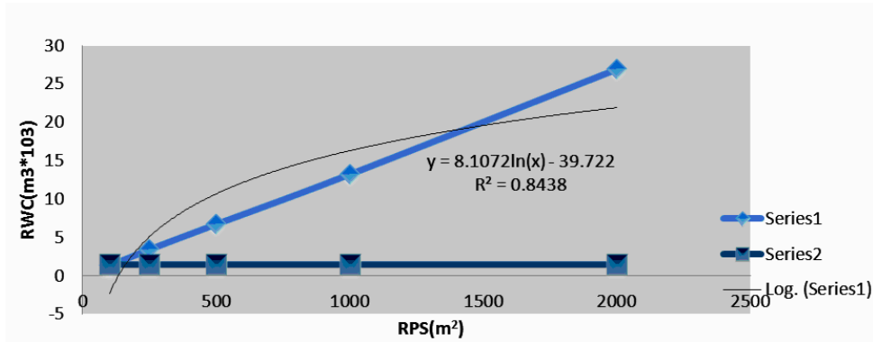
Figure 1. Calibration measures for Rainwater collected with constant rainfall depth (1430 mm) under five Roof plan size in 1996.
