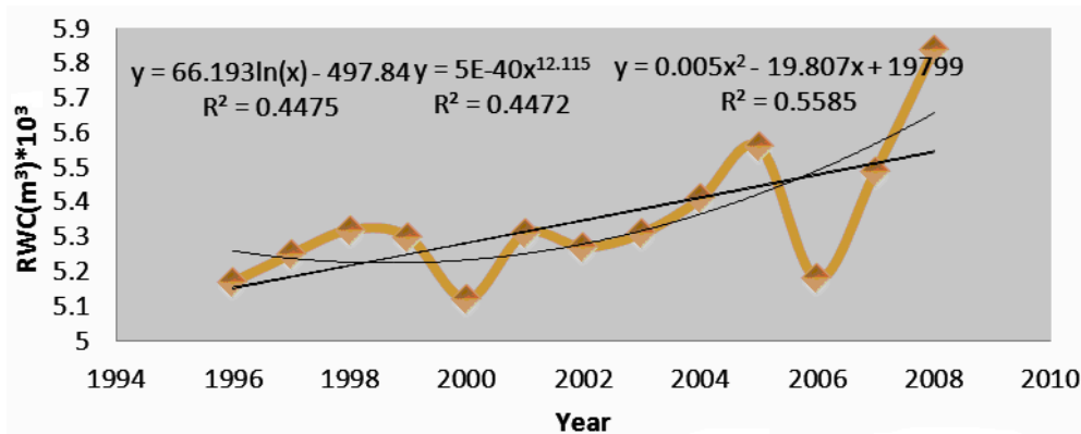
Figure 4. Average volume of rainwater collected at selected areas in Auchi
