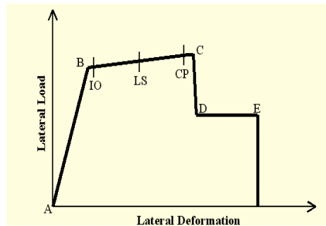
Figure 2. Lateral load Vs Deformation
