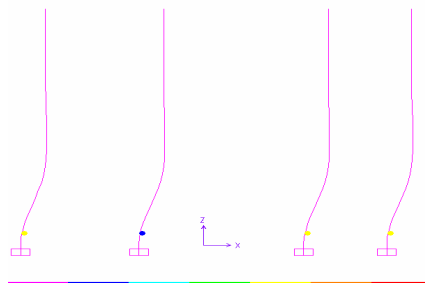
Figure 10. Deformed shape at step 4
