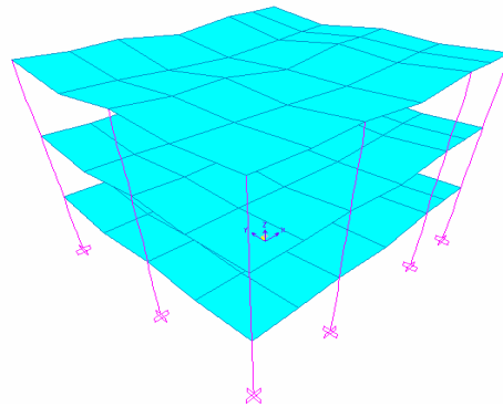
Figure 2. Deformed shape (DEAD)
