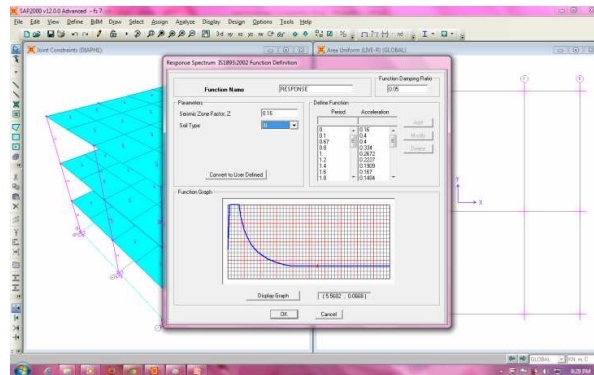
Figure 3. Response spectrum
