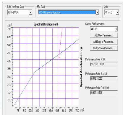
Figure 4. Pushover curve
