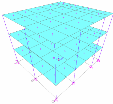
Figure 3. 3-D View
