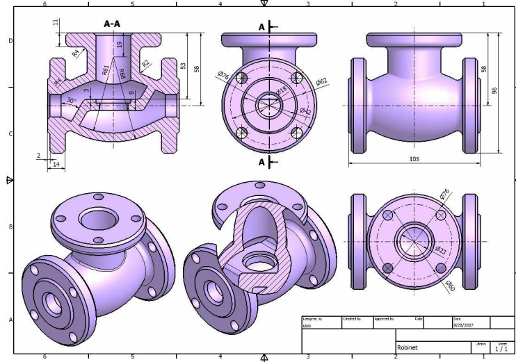
Figure 1. The main dimensions of the admission valve
