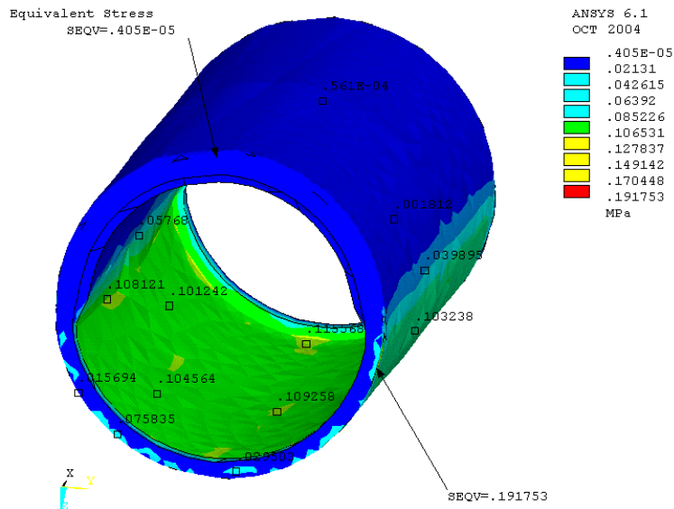
Figure 11 Equivalent stress for first loading case
