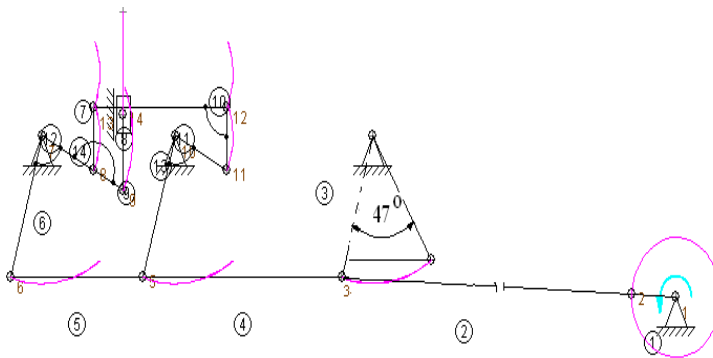
Figure 3 Cinematic scheme and couple trajectory adequate by one complete rotation of crank
