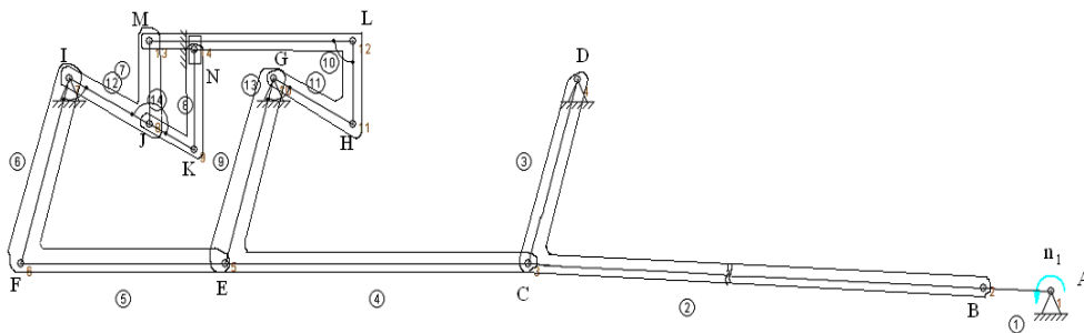
Figure 2 Structural decomposition of mechanism
