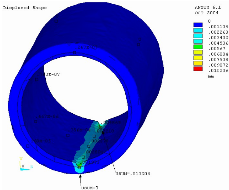
Figure 14 Displaced shape for second loading case
