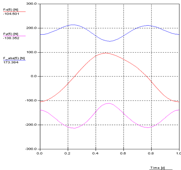
Figure 8 Force variation in node 5
