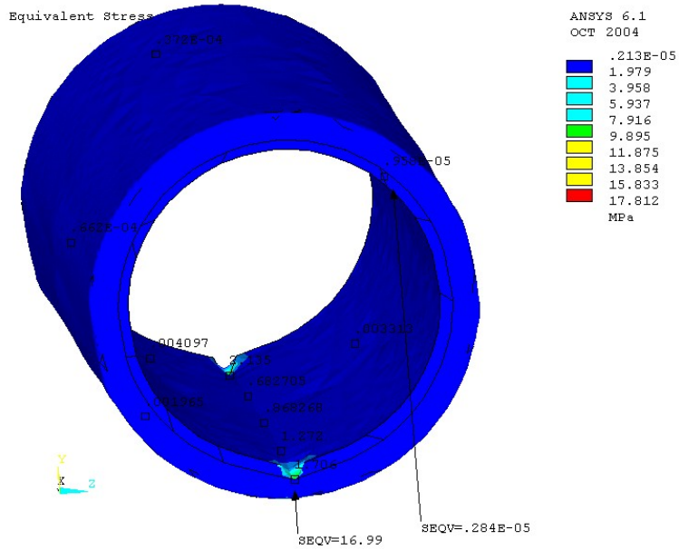
Figure 12 Equivalent stress for second loading case
