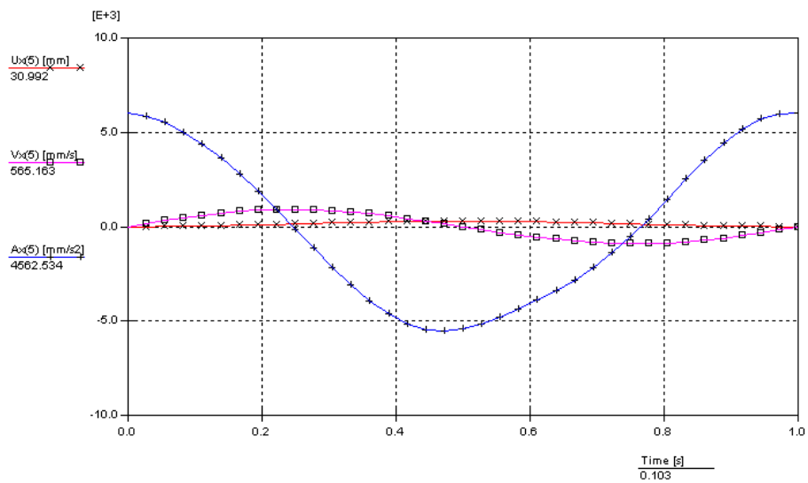
Figure 5 The time dependent variation of space, speed and acceleration for node 5, on the OX axe
