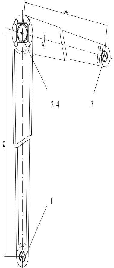
Figure 1 Subensemble of first wire brake mechanism 1,2,3,4 – bronze bushes
