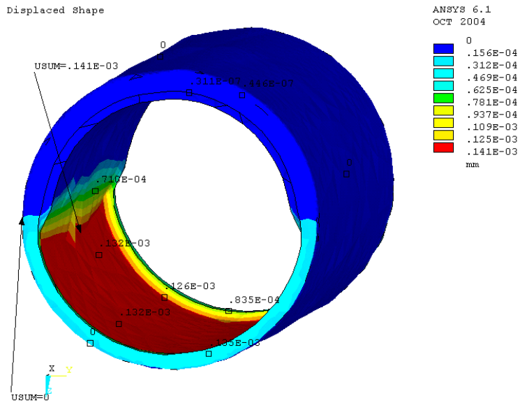
Figure 13 Displaced shape for first loading case
